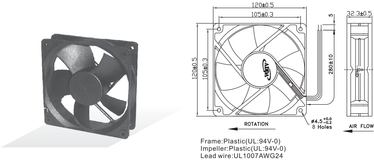
External Dimensions
